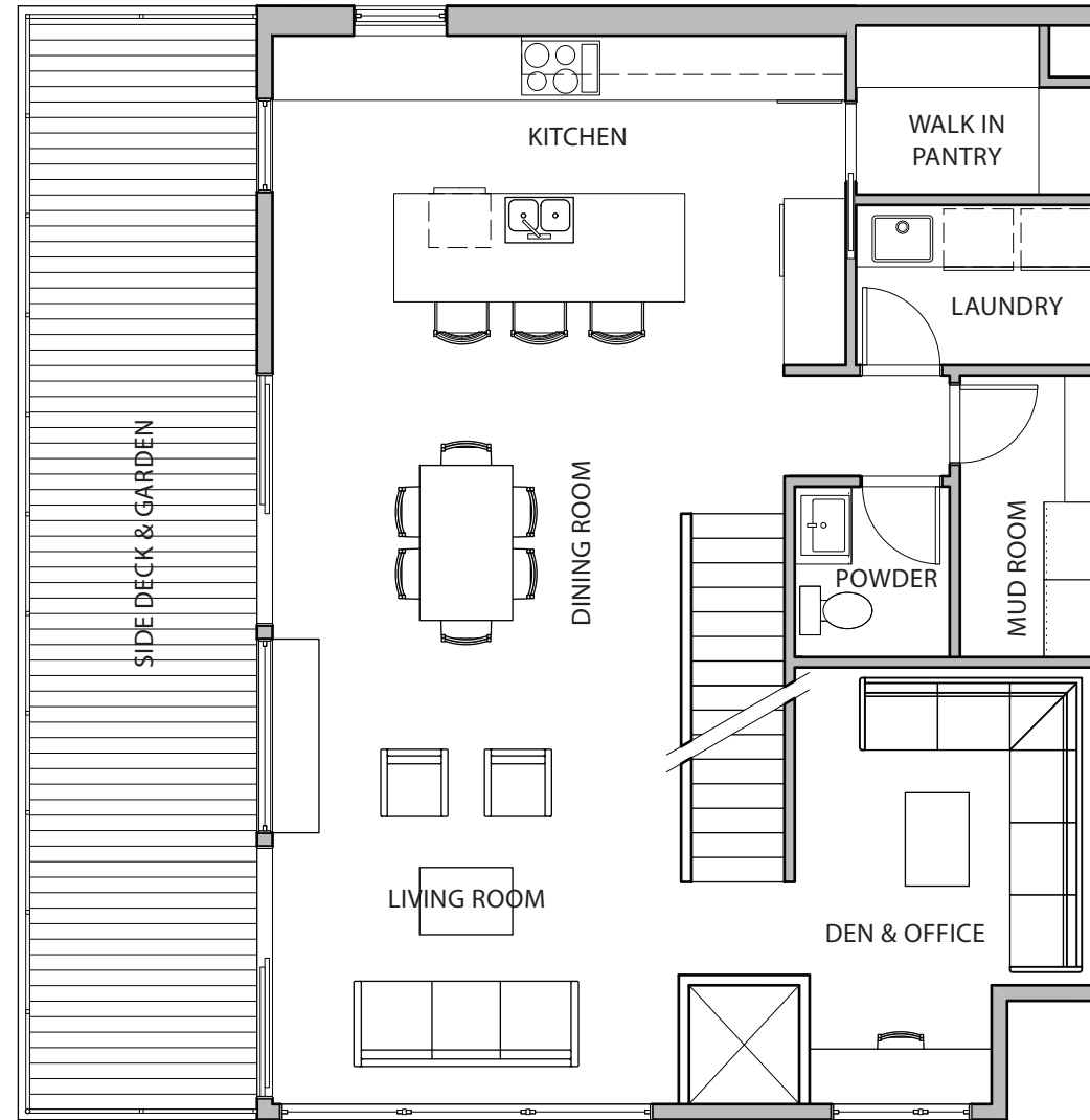
Liveable: 978 sq ft Amenity: 277 sq ft
